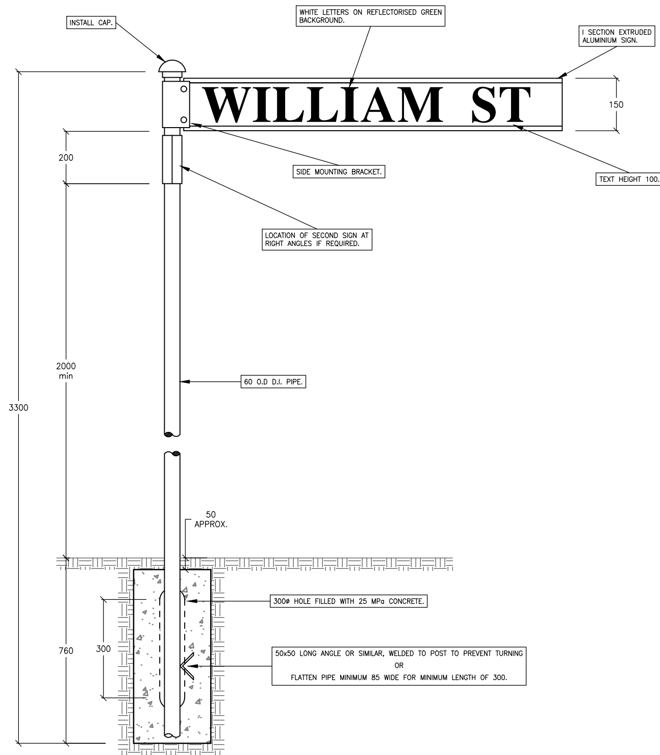
STANDARD DETAIL NOT TO SCALE
